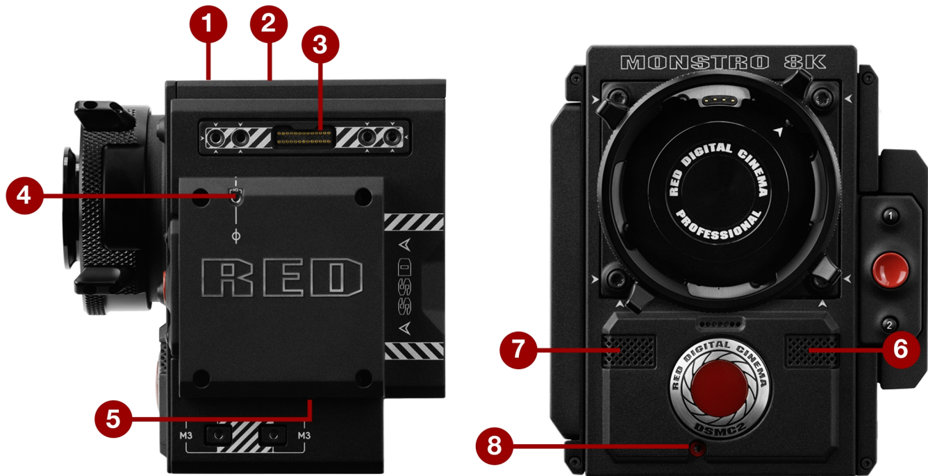
Figure: DSMC2 MONSTRO Ports and Features
